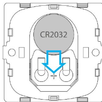
Figure 1: Inserting battery
